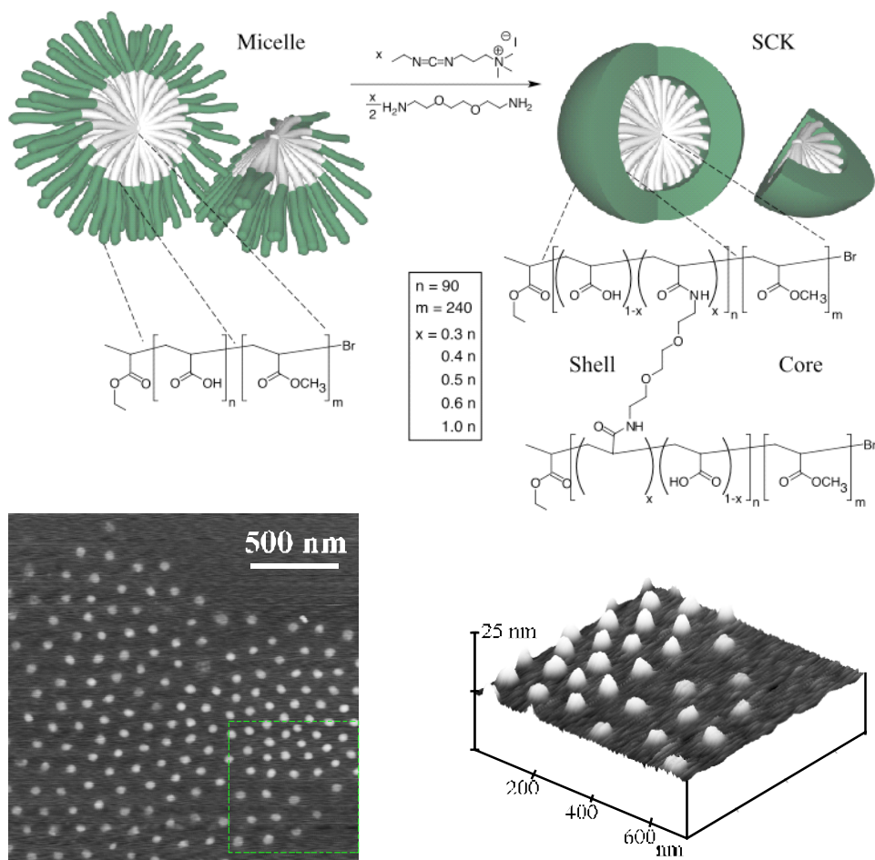
FIGURE 4.17 Polymer micelles can be formed by noncovalent interactions. Top : The shell can be chemically crosslinked to stabilize the nanoparticles. Bottom : Atomic force microscopy displays the nanoparticle shape and size. SOURCE: Karen L. Wooley, Washington University, St. Louis, Mo.
